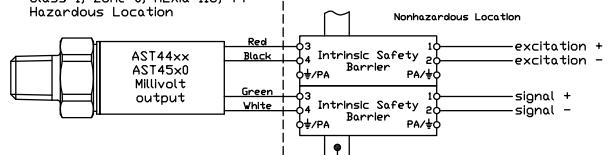
Figure 1: Wiring diagram for 4-wire, mV output
